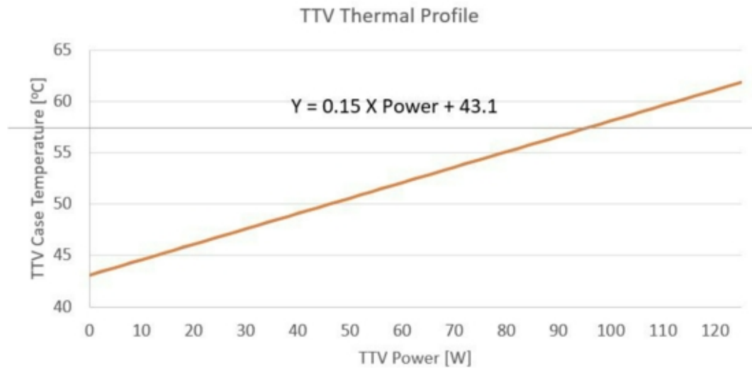
Thermal Profile for PCG 2020A Processor
