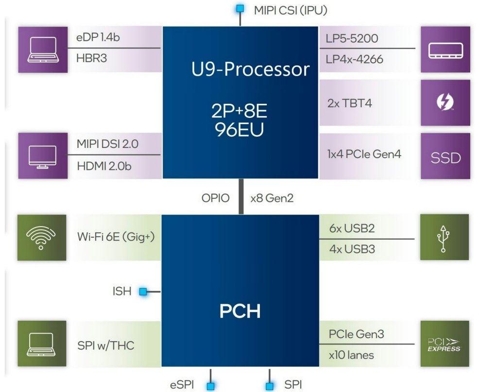
U9 Processor Line Platform Diagram
