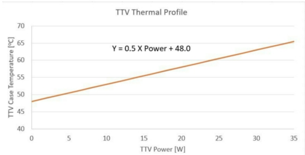
Thermal Test Vehicle Thermal Profile for PCG 2020D Processor
