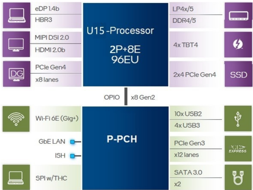
U15 Processor Line Platform Diagram
