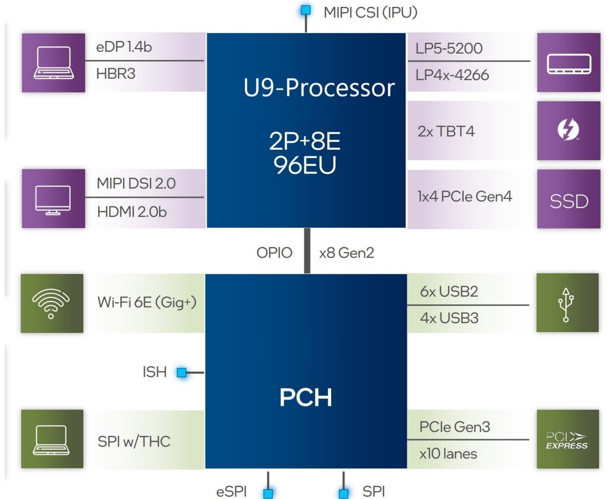
U9 Processor Line Platform Diagram
