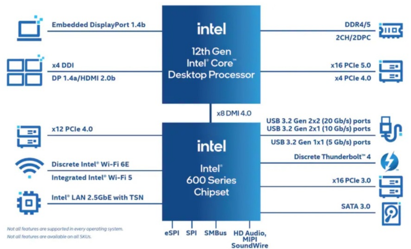
S Processor Line Platform Diagram
