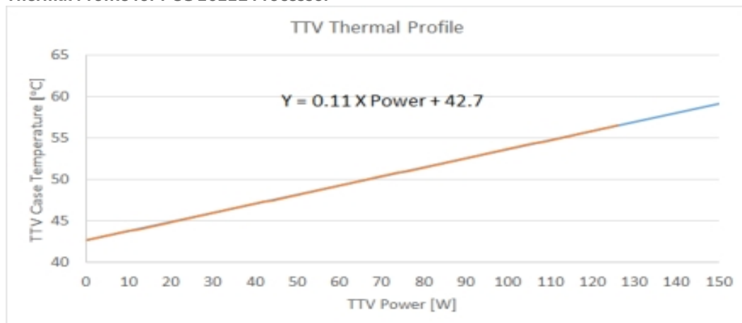
Thermal Profile for PCG 2022E Processor
