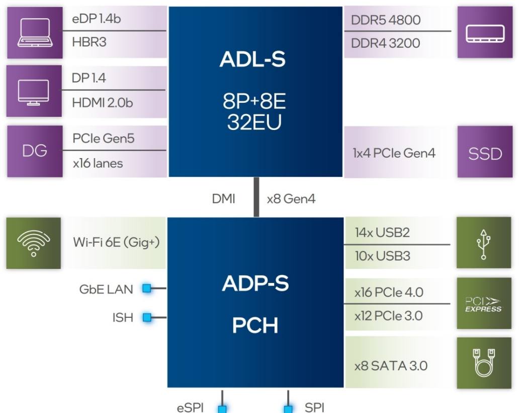
HX Processor Line Platform Diagram
