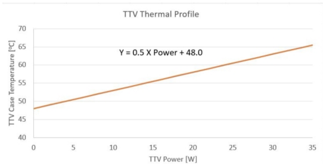
Thermal Test Vehicle Thermal Profile for PCG 2020D Processor
