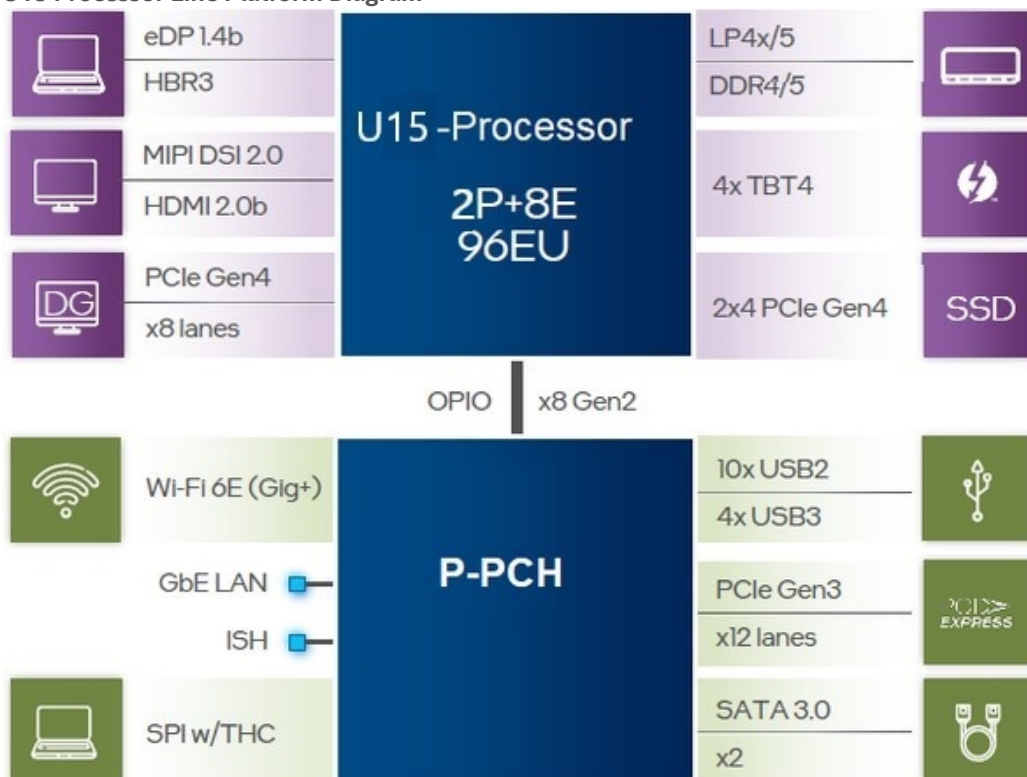
U15 Processor Line Platform Diagram
