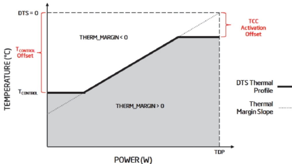
Digital Thermal Sensor (DTS) 2.0 Definition Points
